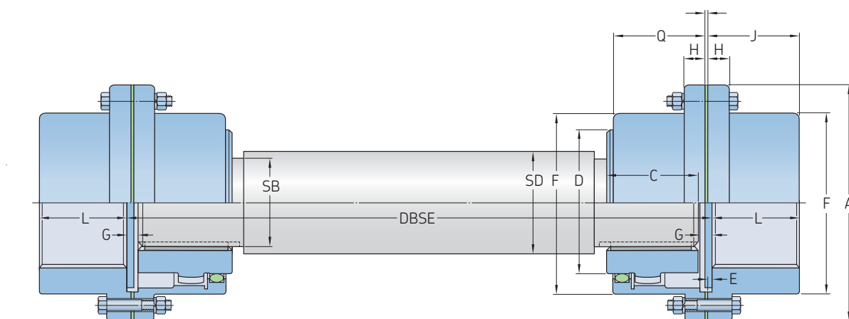
Flex hub on floating shaft
